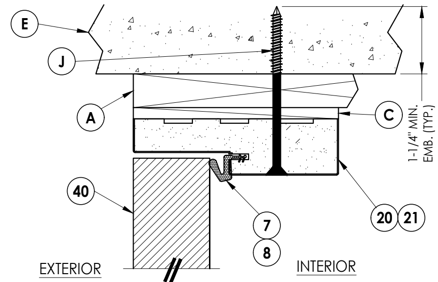
2 VERTICAL CROSS SECTION 6 Outswing shown - inswing also approved Shown w/1X sub-buck
